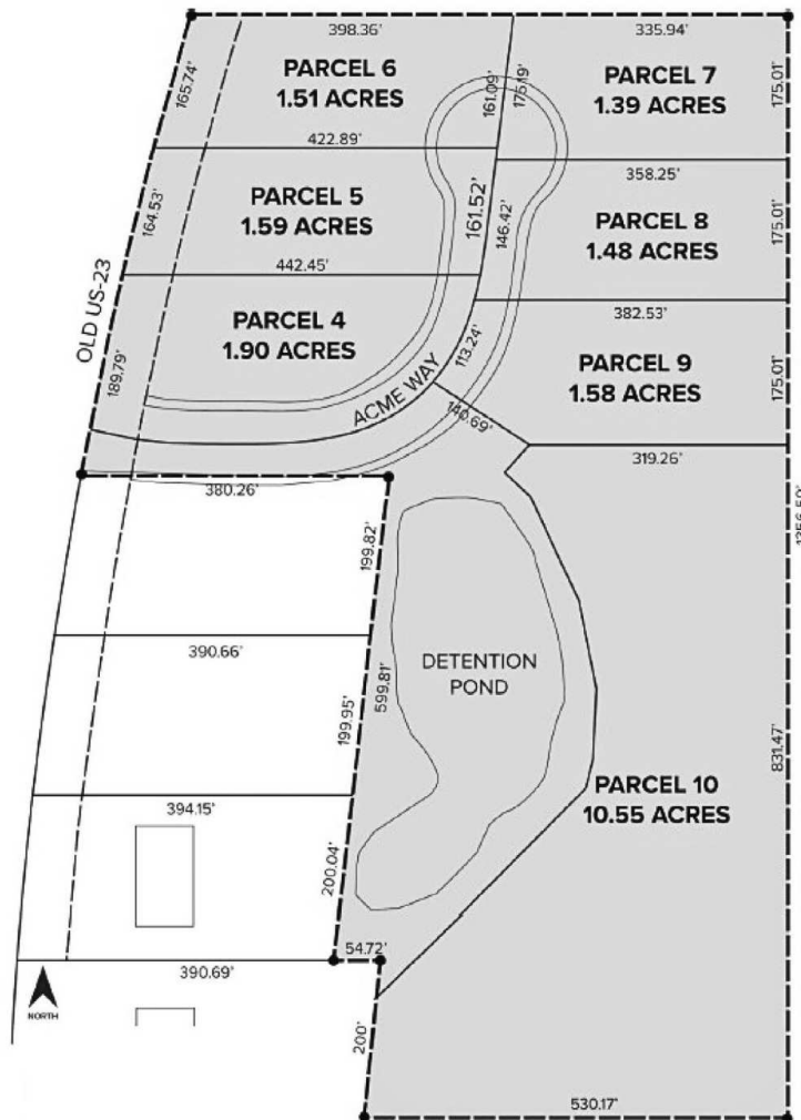
Site Plan
